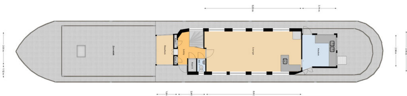
Bovendek Boathouse 2
